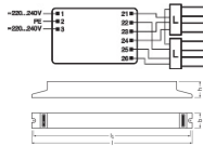
Scheda tecnica Osram LED Driver QuickTronic professional DL 2X55 GII
